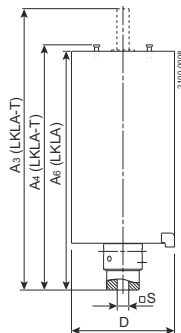
Figure 17. With coupling
