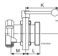
Figure 15. LKB with male part/nut and liner
