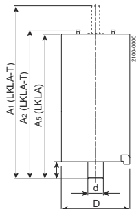
Figure 16. Without coupling
