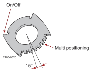
Figure 3. Positioning cap
