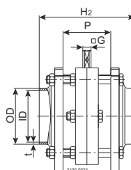
Figure 14. c. LKB-F with welding ends
